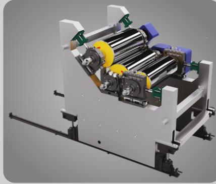
Calendar Unit
